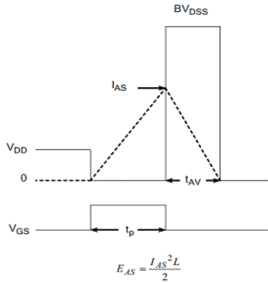
Figure21.Unclamped Inductive Switching
