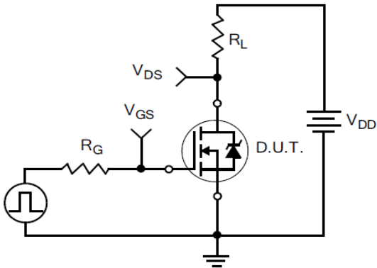
Figure 16. Resistive Switching Test Circuit Waveforms
