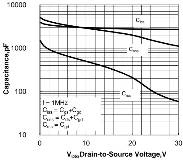
Figure 12. Capacitance Characteristics
