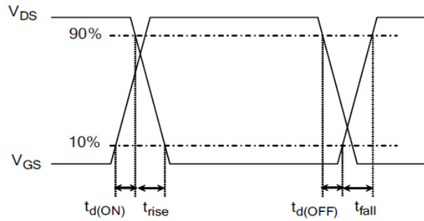
Figure 17. Resistive Switching
