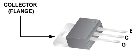
JEDEC TO-220AB (ALTERNATE VERSION)
