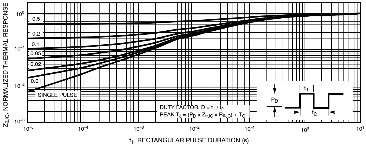
Figure 15. IGBT NORMALIZED TRANSIENT THERMAL RESPONSE, JUNCTION TO CASE
