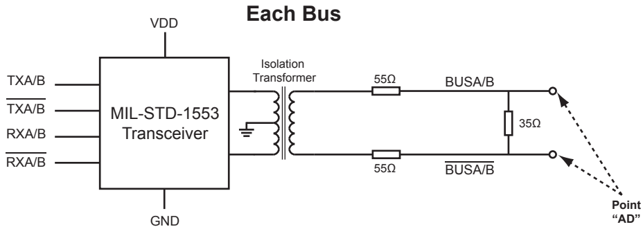
Figure 28. MIL-STD-1553 Direct Coupled Test Circuits
