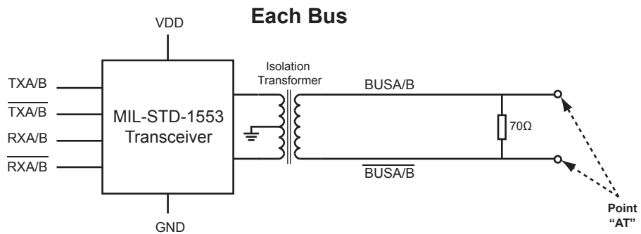
Figure 29. MIL-STD-1553 Transformer Coupled Test Circuits
