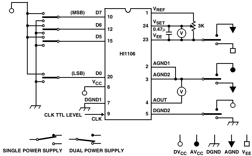
FIGURE 1. DC CHARACTERISTICS
