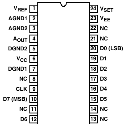
HI1106 (PDIP, SOIC) TOP VIEW
