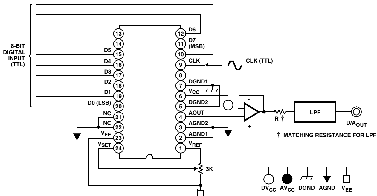
FIGURE 21. DUAL POWER SUPPLY
