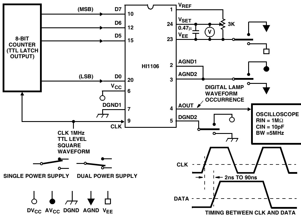
FIGURE 4. GLITCH AREA
