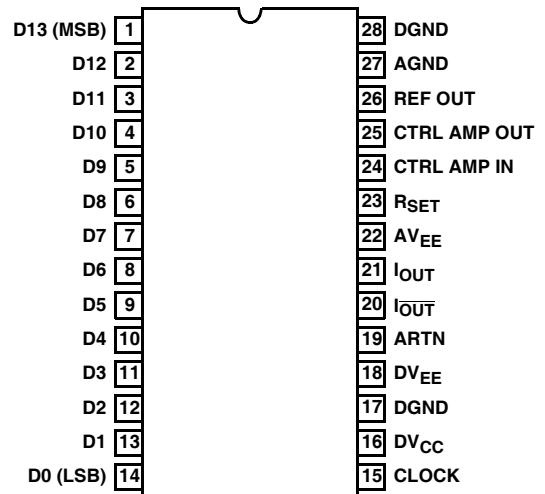
HI5741 (28 LD SOIC) TOP VIEW
