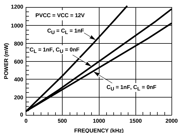
FIGURE 2. 1nF LOADING PROFILE
