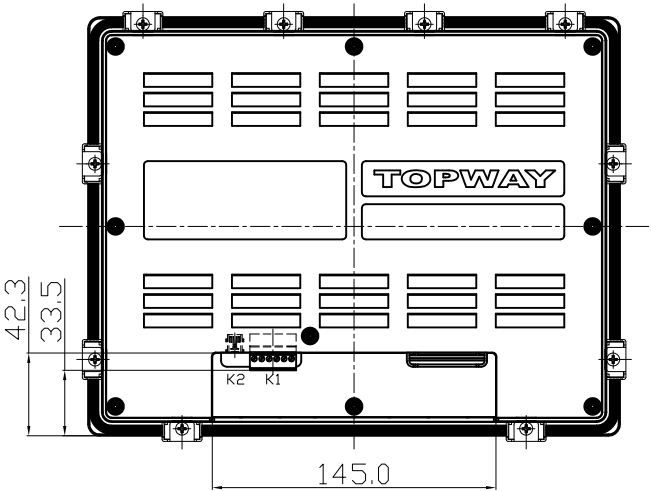
REAR VIEW Scale=1/4
