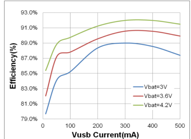
Figure 16. Boost Efficiency
