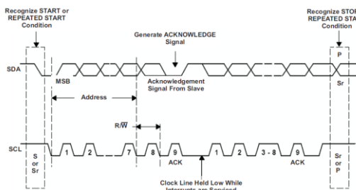
Figure 22. Bus Protocol
