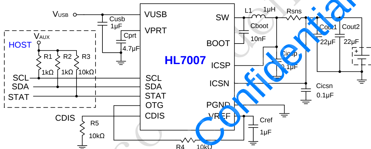
Figure 1. HL7007 Typical Application Diagram
