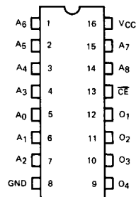
PIN NAMES
