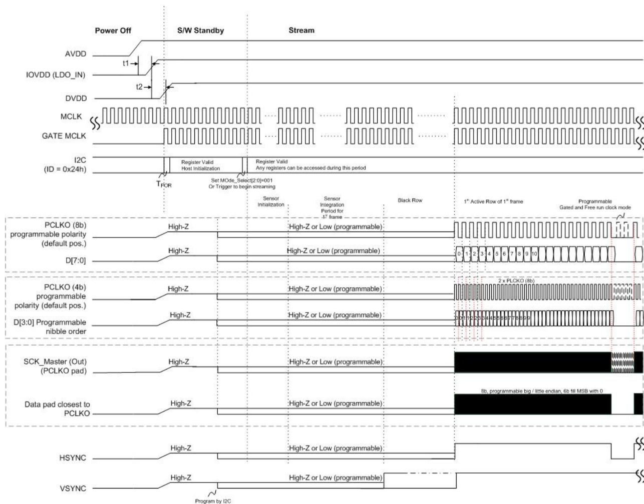
Figure 1.2: Power up sequence
