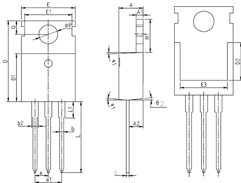
TO-220
