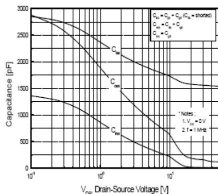
Figure 5. Capacitance Characteristics
