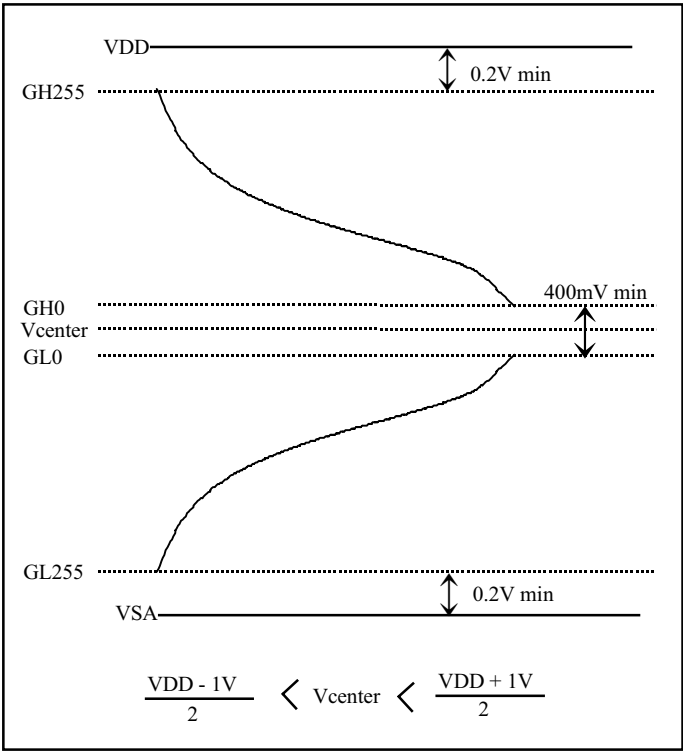
[Fig 5] Reference voltage electrical characteristics
