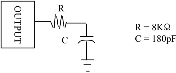
[Fig 6] Load conditions of analog output pin. The values of R and C could be changed according to the situation.
