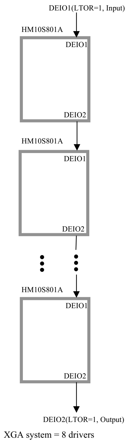
[Fig 4] Output driver control inputs
