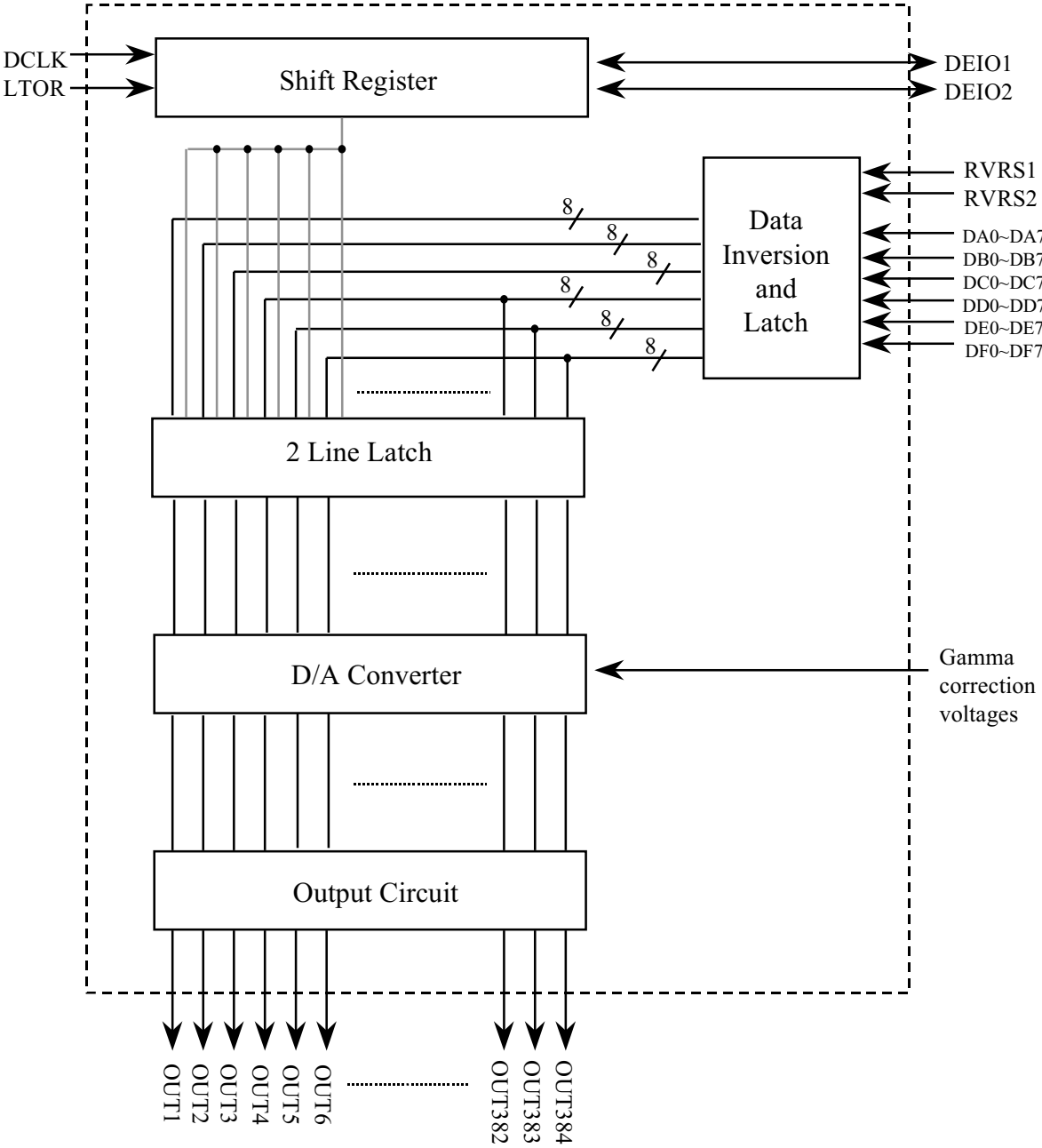
[Fig 1] Block diagram of HM10S801A
