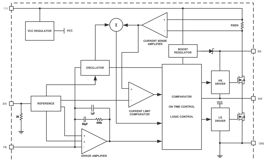
Figure 2. HM1484D Block Diagram
