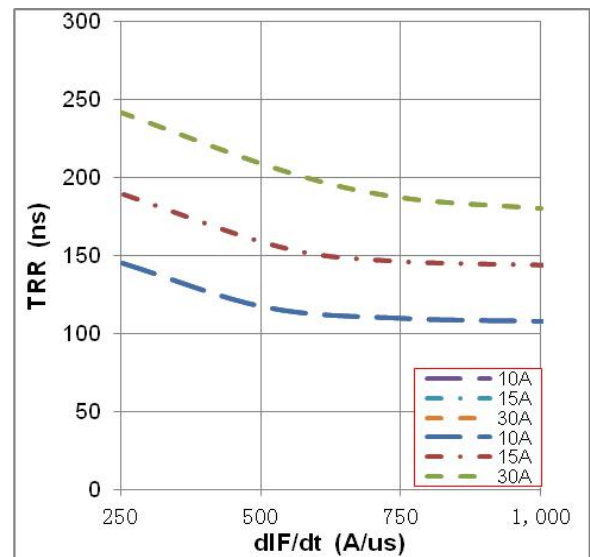
Figure16: typical diode TRR VS. dIF/dt,
