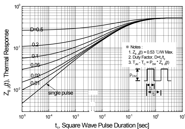
Figure 11-1. Transient Thermal Response Curve for HM16N50
