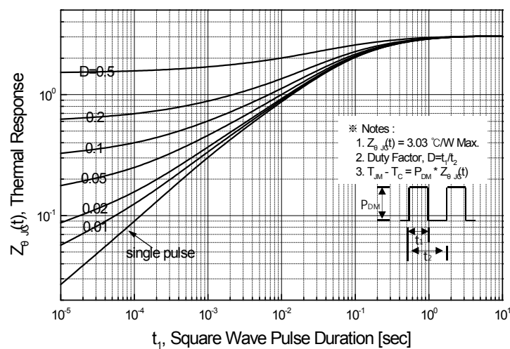
Figure 11-2. Transient Thermal Response Curve for HM16N50F
