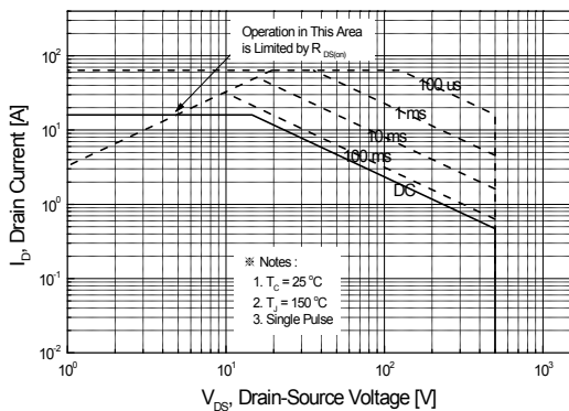
Figure 9-1. Maximum Safe Operating Area for HM16N50
