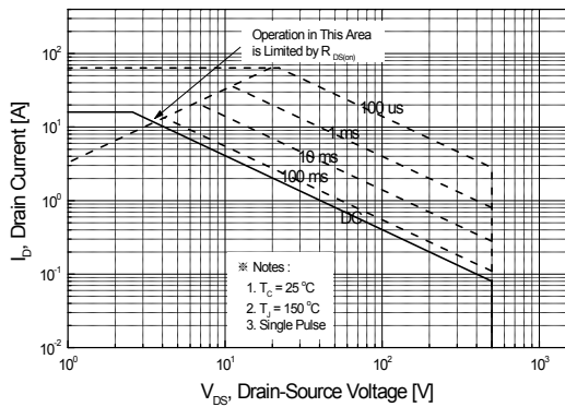
Figure 9-2. Maximum Safe Operating Area for HM16N50F
