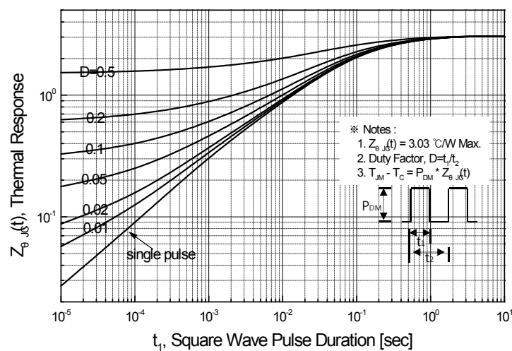
Figure 11-2. Transient Thermal Response Curve for HM18N50F
