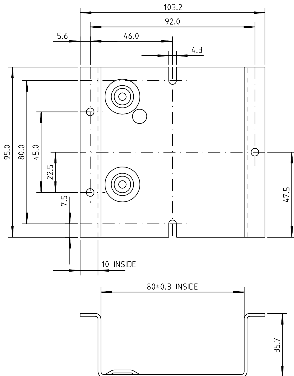
Fig.2 HM199 Dimensions.
