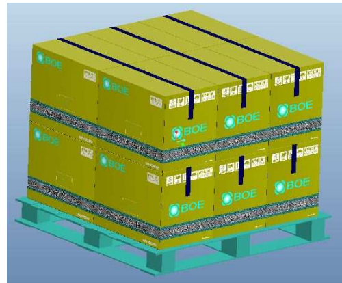
Wrap the Pallet Assy loaded 1story, 2stories from downside through side and to edge of upside. (12Boxes/Pallet)
