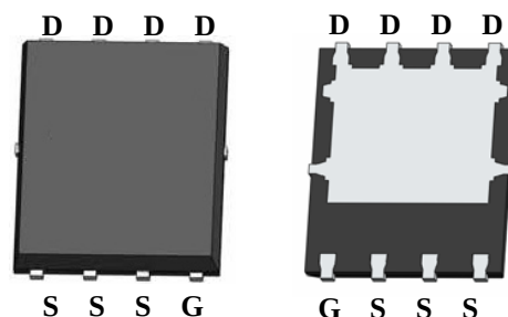
DFN5X6-8L top view
