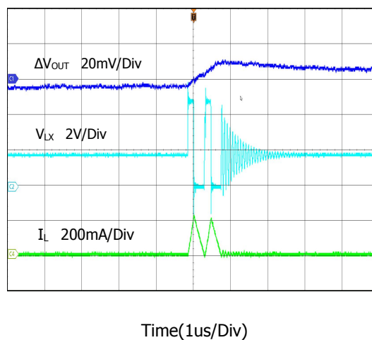
Output Ripple
