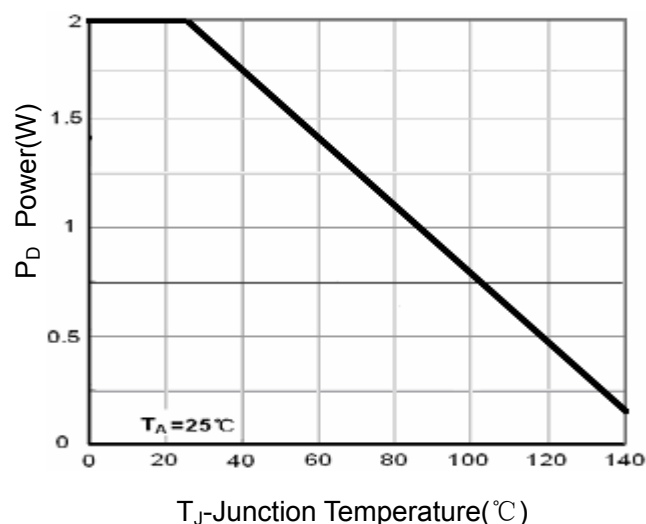
Figure 8 Power Dissipation
