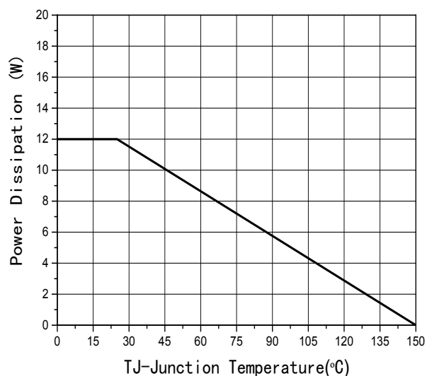
Fig7 Power De-rating
