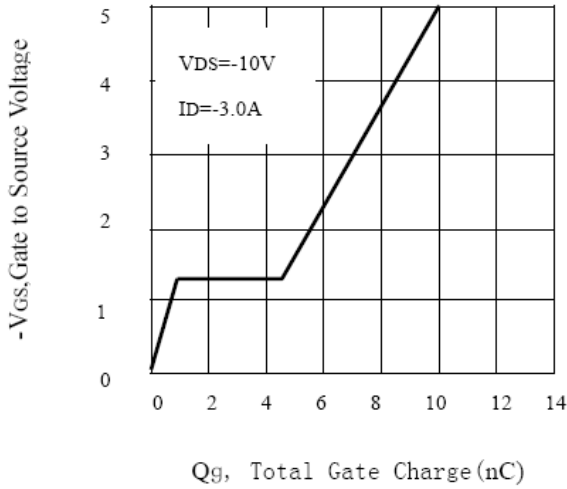
Figure9. Gate Charge
