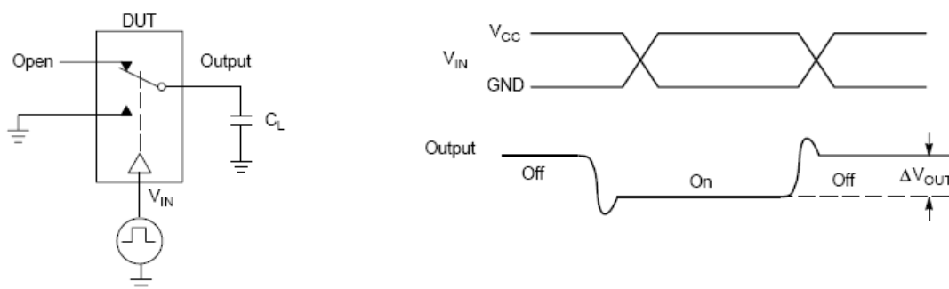
Figure3: Charge Injection
