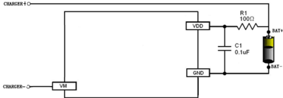
Fig 6 HM5433G in a Typical Battery Protection Circuit
