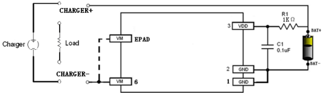
Fig 6 HM5493A in a Typical Battery Protection Circuit
