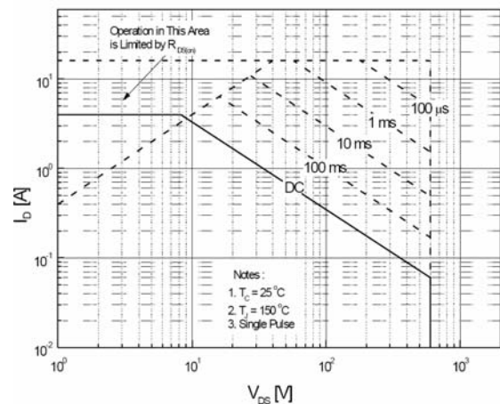
Maximum Safe Operating Area For HM5N60F
