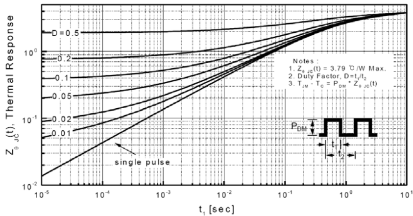
Transient Thermal Response Curve For HM5N60F
