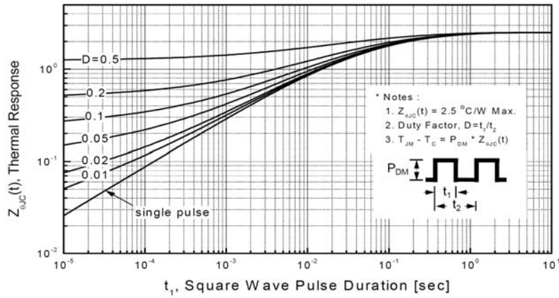
Transient Thermal Response Curve For HM5N60
