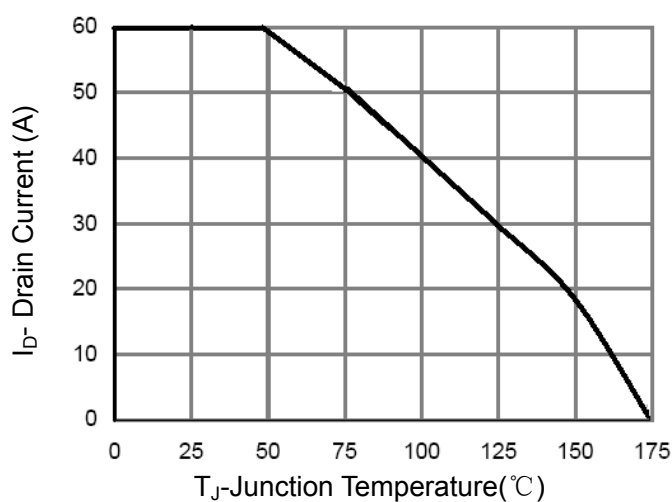
Figure 9 ID De-rating
