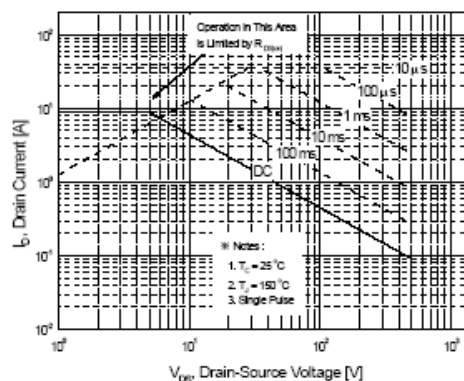
Figure 9-2. Maximum Safe Operating Area for HM840F
