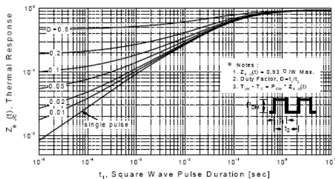
Figure 11-1. Transient Thermal Response Curve for HM840
