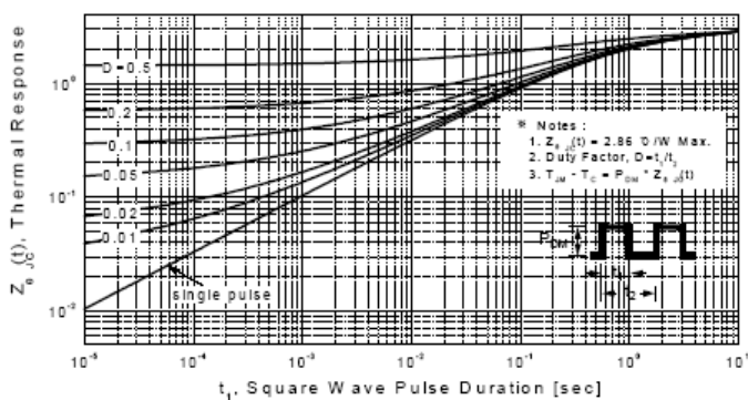
Figure 11-2. Transient Thermal Response Curve for HM840F
