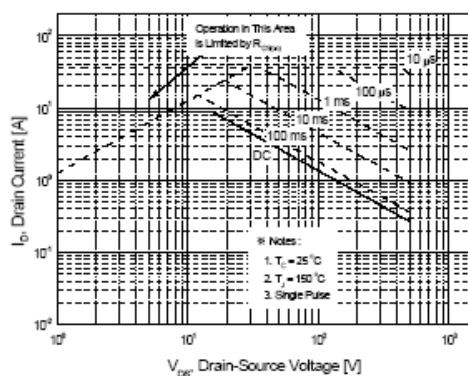
Figure 9-1. Maximum Safe Operating Area for HM840
