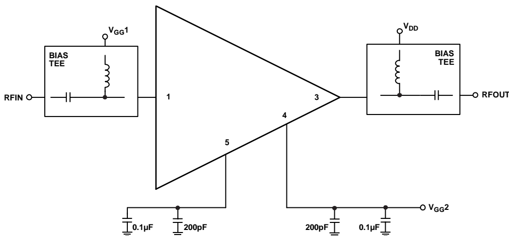
Figure 23. Suggested Alternate Applications Circuit
