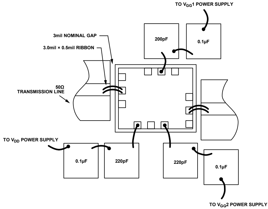
Figure 24. Assembly Diagram
