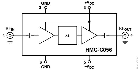
Figure 2. Pin Configuration
