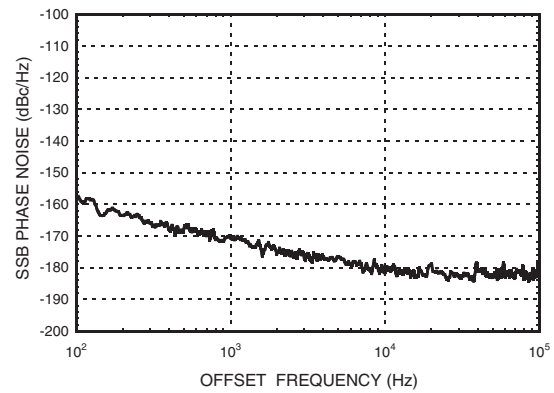
Phase Noise at Pout = Psat @ 9 GHz
