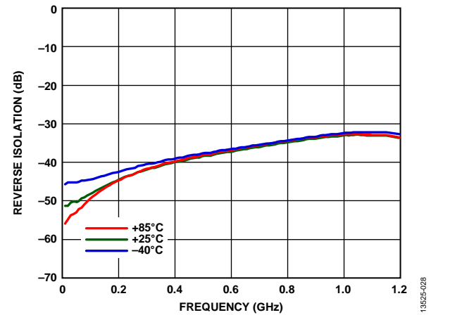
Figure 28. Reverse Isolation vs. Frequency at Various Temperatures
