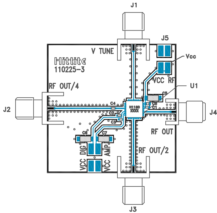
Figure 16. Evaluation Board
