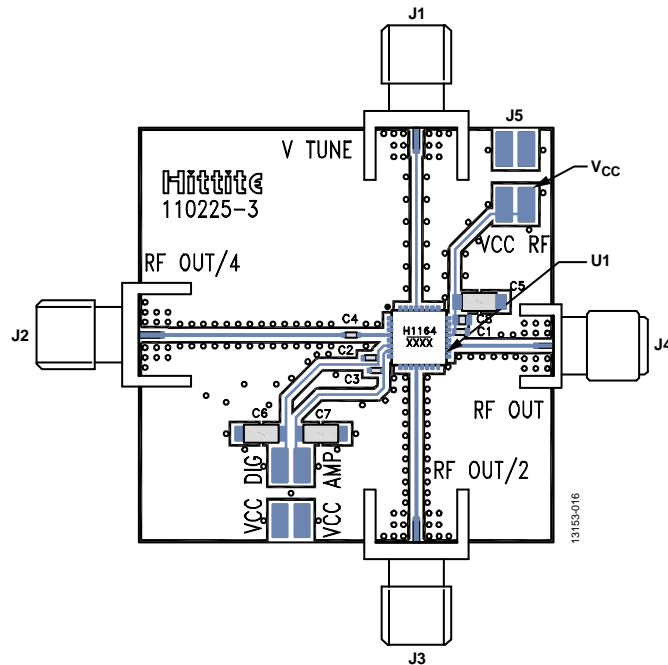
Figure 16. 110225-3 Evaluation PCB
