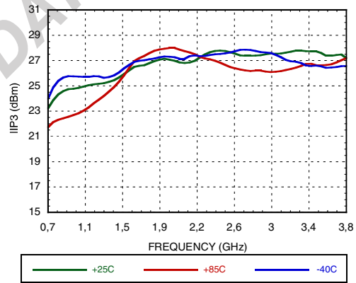
Figure 22. High Side LO Input IP3 vs. Frequency @ VGATE=5V [2]
