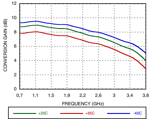
Figure 19. Low Side LO Conversion Gain vs. Frequency @ VGATE=5V [1][2]
