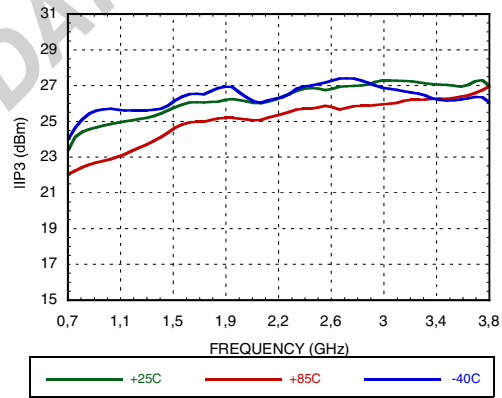
Figure 28. High Side LO Input IP3 vs. Frequency @ VGATE=4.9V[2]
