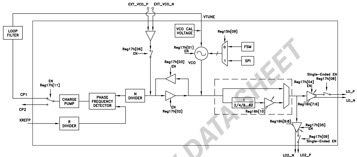
Figure 66. HMC1190ALP6NE PLL VCO Block Diagram
