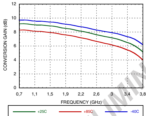
Figure 33. High Side LO Conversion Gain vs. Frequency @ VGATE=4.8V [1][2]
