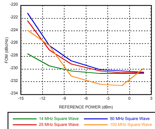
Figure 59. Reference Input Sensitivity, Square Wave, 50 Ω [3]
