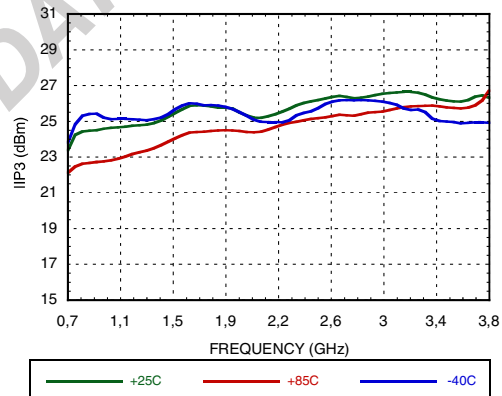
Figure 34. High Side LO Input IP3 vs. Frequency @ VGATE=4.8V[2]
