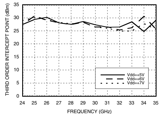
IP3 vs. Vdd
