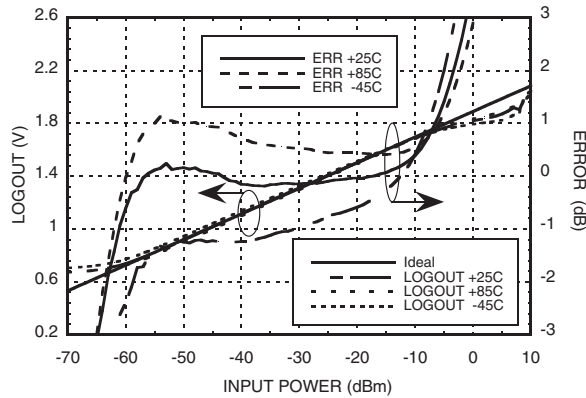
LOGOUT Voltage & Error vs. Input Power, F_{in} = 1900 \text{ MHz}
