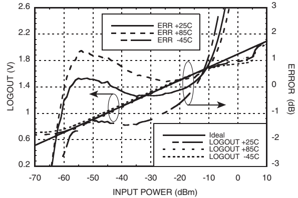
LOGOUT Voltage & Error vs. Input Power, F_{in} = 2500 \text{ MHz}
