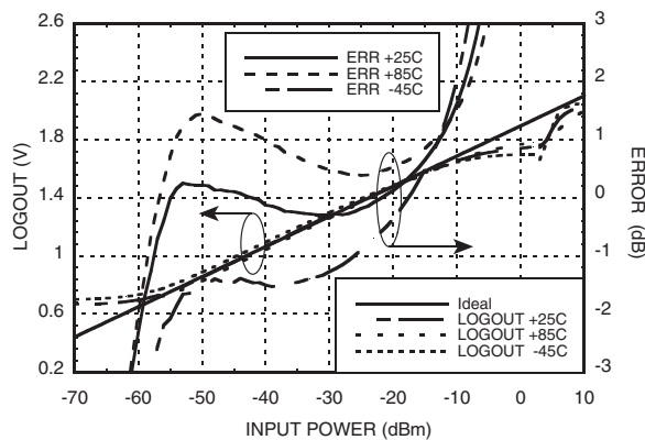
LOGOUT Voltage & Error vs. Input Power, F_{in} = 3000 \text{ MHz}
