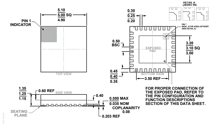
Figure 71. 32-Lead Lead Frame Chip Scale Package, Premolded Cavity [LFCSP_CAV] 5 mm x 5 mm Body and 1.25 mm Package Height (CG-32-2) Dimensions shown in millimeter
