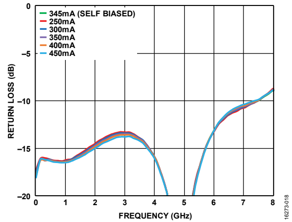
Figure 18. Input Return Loss vs. Frequency for Various Supply Currents ( I_{DD} ), Externally Biased Mode, V_{DD} = 12 V, V_{GG2} = Open, Controlled V_{GG1}
