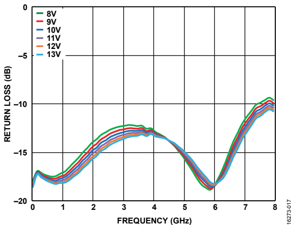
Figure 17. Output Return Loss vs. Frequency for Various Supply Voltages ( V_{DD} ), Self Biased Mode, V_{GG2} = 5 V, V_{GG2} = Open, V_{GG1} = GND
