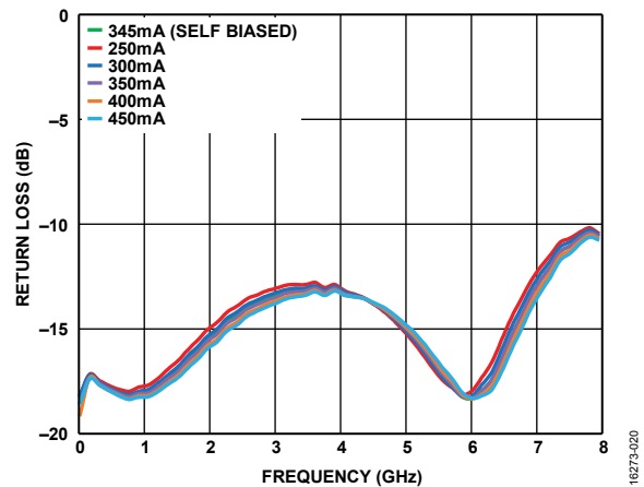
Figure 20. Output Return Loss vs. Frequency for Various Supply Currents ( I_{DD} ), External Biased condition, V_{DD} = 12 V, V_{GG2} = Open, Controlled V_{GG1}
