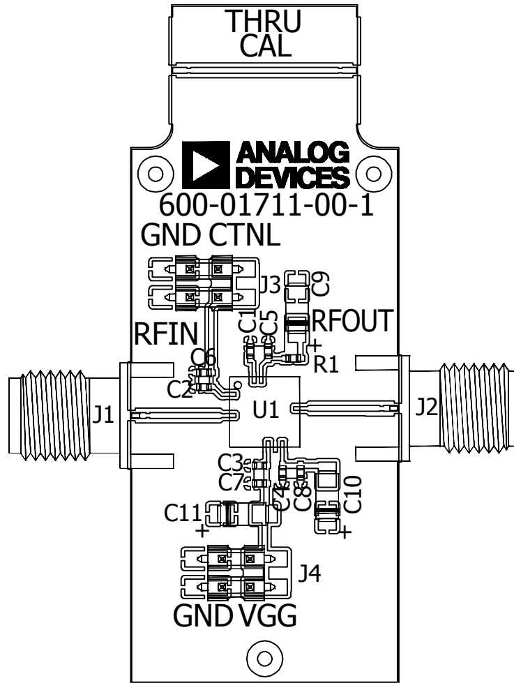
Figure 70. Evaluation PCB
