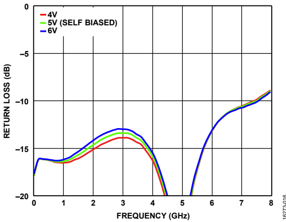
Figure 16. Input Return Loss vs. Frequency for Various V_{GG2} Values, V_{DD} = 12 V, V_{GG1} = GND
