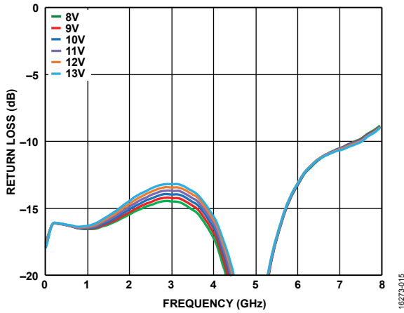
Figure 15. Input Return Loss vs. Frequency for Various Supply Voltages ( V_{DD} ), Self Biased Mode, V_{GG2} = Open, V_{GG1} = GND
