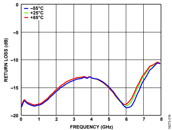
Figure 19. Output Return Loss vs. Frequency for Various Temperatures, Self Biased Mode, V_{DD} = 12 V, V_{GG2} = Open, V_{GG1} = GND
