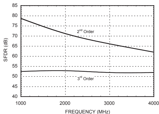
Dual Rank Track-Mode Two-Tone SFDR vs. Frequency [2]
