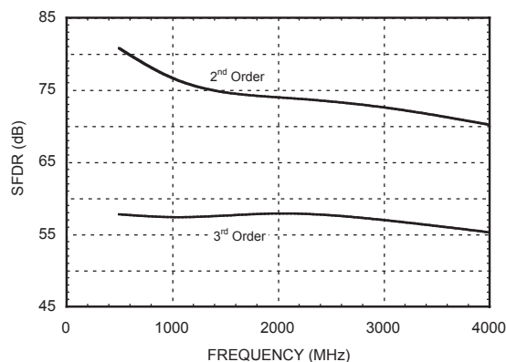
Track-Mode Two-Tone SFDR vs. Frequency [2]
