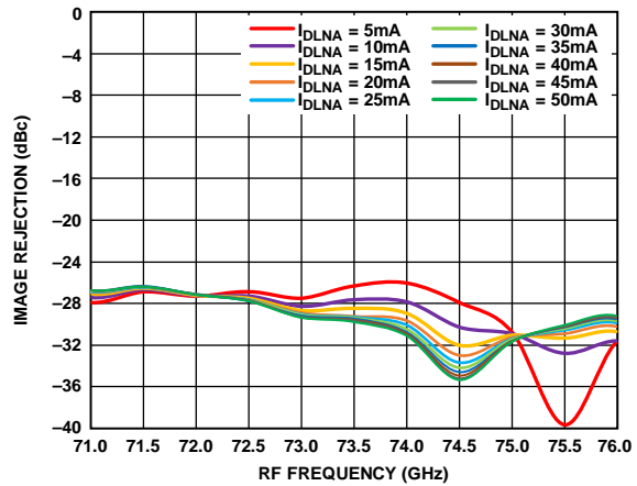
Figure 55. Image Rejection vs. RF Frequency at Various I_{DLNA} Values, RFIN = -20\text{ dBm} , LO = 2\text{ dBm} , IF = 500\text{ MHz} , V_{DLNA} = 3\text{ V}
