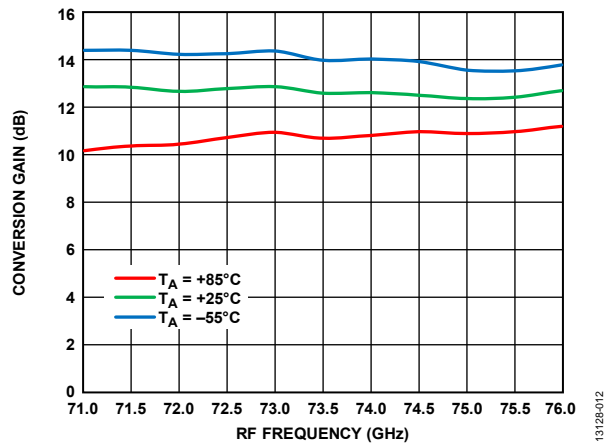
Figure 12. Conversion Gain vs. RF Frequency at Various Temperatures, RFIN = -20 dBm, LO = 2 dBm, IF = 1000 MHz, VDLNA = 3 V
