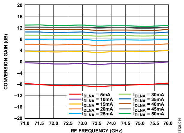
Figure 14. Conversion Gain vs. RF Frequency at Various IDLNA Values, RFIN = -20 dBm, IF = 1000 MHz, VDLNA = 3 V
