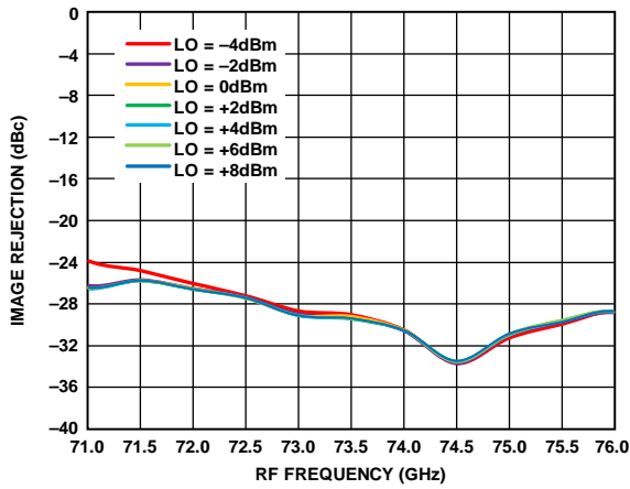
Figure 51. Image Rejection vs. RF Frequency at Various LO Powers, RFIN = -20\text{ dBm} , IF = 500\text{ MHz} , V_{DLNA} = 4\text{ V}
