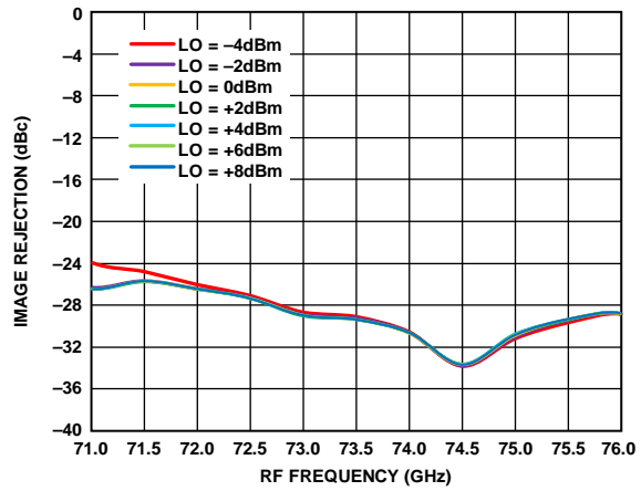
Figure 54. Image Rejection vs. RF Frequency at Various LO Powers, RFIN = -20\text{ dBm} , IF = 500\text{ MHz} , V_{DLNA} = 3\text{ V}
