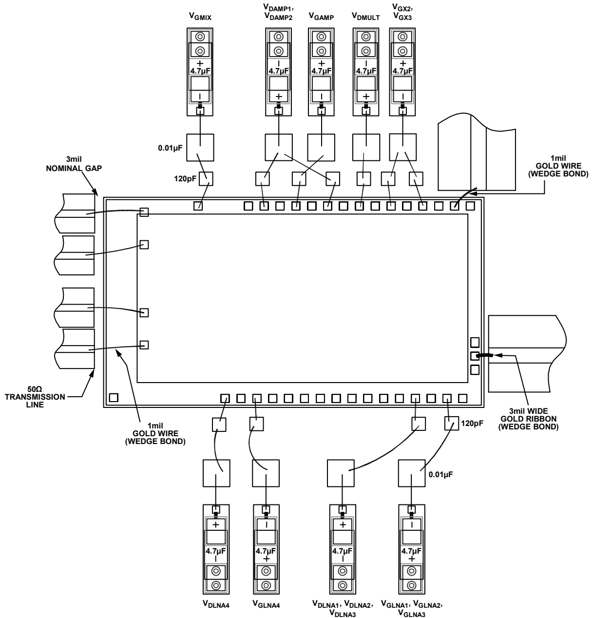
Figure 213. Assembly Diagram
