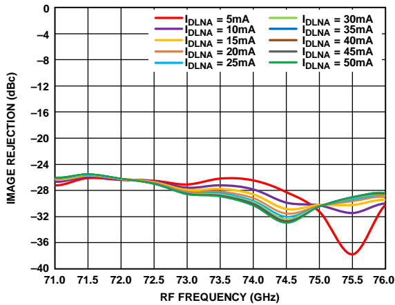
Figure 52. Image Rejection vs. RF Frequency at Various I_{DLNA} Values, RFIN = -20\text{ dBm} , LO = 2\text{ dBm} , IF = 500\text{ MHz} , V_{DLNA} = 4\text{ V}
