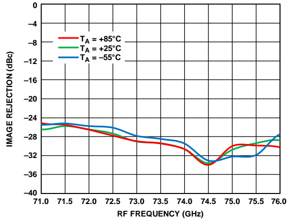
Figure 53. Image Rejection vs. RF Frequency at Various Temperatures, RFIN = -20\text{ dBm} , LO = 2\text{ dBm} , IF = 500\text{ MHz} , V_{DLNA} = 3\text{ V}
