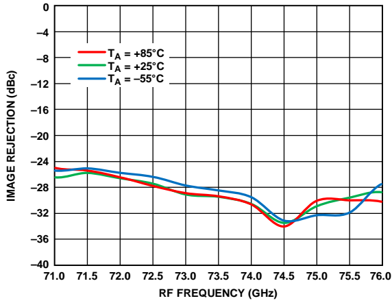
Figure 50. Image Rejection vs. RF Frequency at Various Temperatures, RFIN = -20\text{ dBm} , LO = 2\text{ dBm} , IF = 500\text{ MHz} , V_{DLNA} = 4\text{ V}
