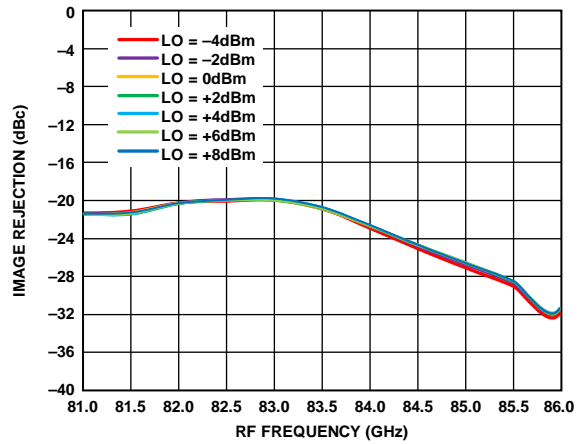
Figure 176. Image Rejection vs. RF Frequency at Various LO Powers, RFIN = -20\text{ dBm} , IF = 2000\text{ MHz} , V_{DLNA} = 3\text{ V}
