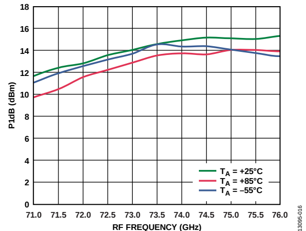
Figure 16. Input P1dB vs. RF Frequency at Various Temperatures, LO = 2 dBm, IF = 1000 MHz, LSB
