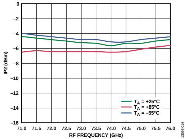
Figure 14. Input IP2 vs. RF Frequency at Various Temperatures, I_{FIN} = 5 dBm, LO = 2 dBm, IF = 1000 MHz, LSB
