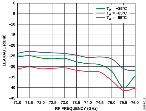
Figure 15. 6x LO Leakage at RFOUT vs. RF Frequency at Various Temperatures, I_{FIN} = 5 dBm, LO = 2 dBm, IF = 1000 MHz, LSB
