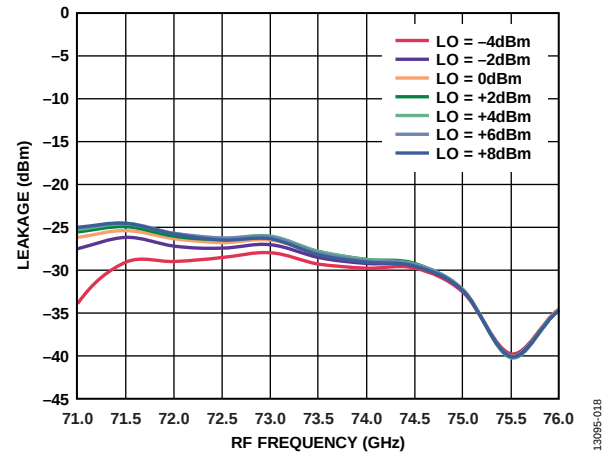
Figure 18. 6x LO Leakage at RFOUT vs. RF Frequency at Various LO Powers, I_{FIN} = 5 dBm, IF = 1000 MHz, LSB
