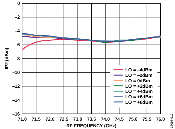
Figure 17. Input IP2 vs. RF Frequency at Various LO Powers, I_{FIN} = 5 dBm, IF = 1000 MHz, LSB
