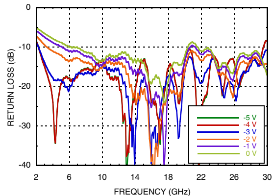
Input Return Loss Vctrl1 = Variable, Vctrl2 = -5V
