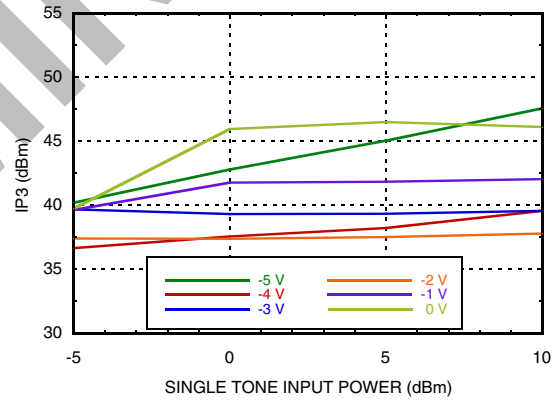
Input IP3 vs Input Power @ 5 GHz Vctrl1 = Variable, Vctrl2 = -5V
