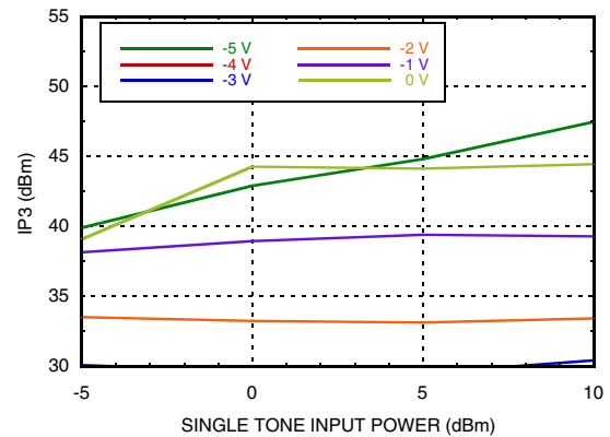
Input IP3 vs Input Power Over Vctrl @ 5 GHz, Vctrl1 = Vctrl2
