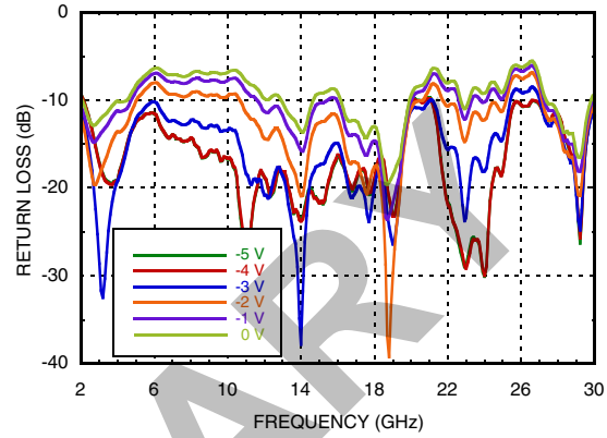
Output Return Loss Vctrl1 = Variable, Vctrl2 = -5V
