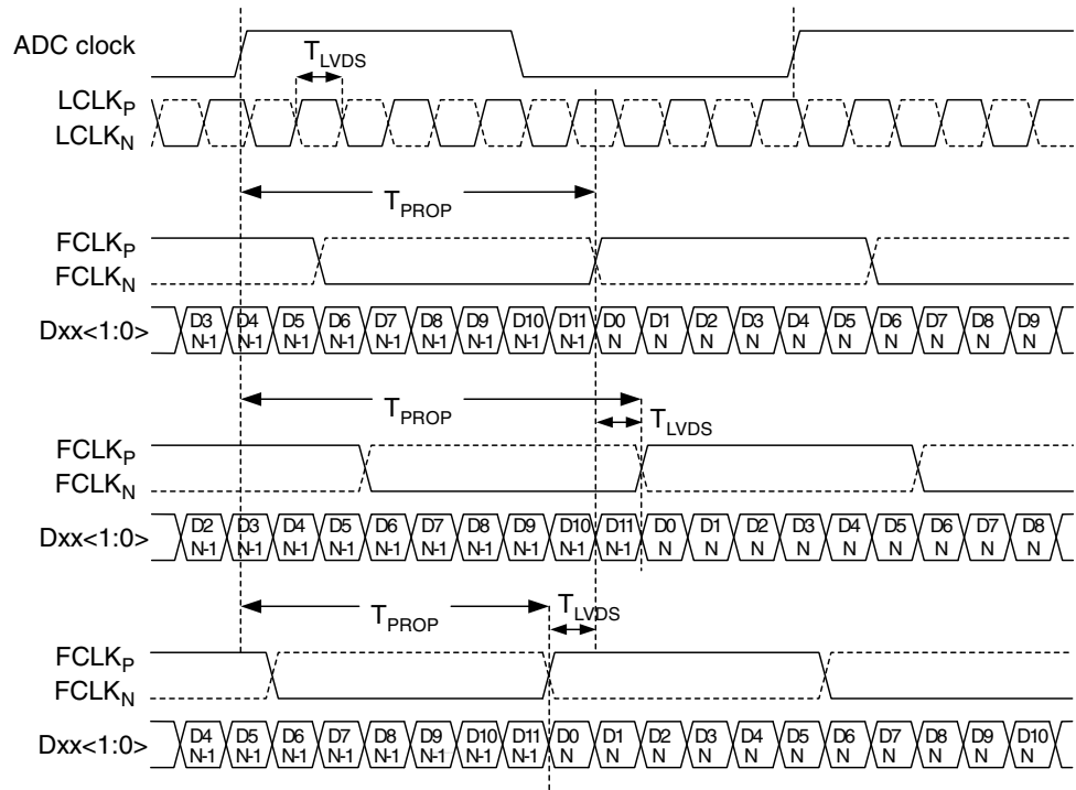
Figure 10. LVDS output timing adjustment
