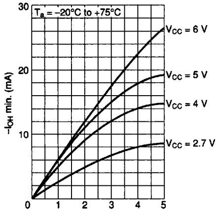
-I_{OH\ min.} vs. (V_{CC} - V_{OH}) characteristics (D 4 to D 15 pins)
