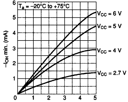
-I_{OH\ min.} vs. (V_{CC} - V_{OH}) characteristics (R0 to R2 ports)
