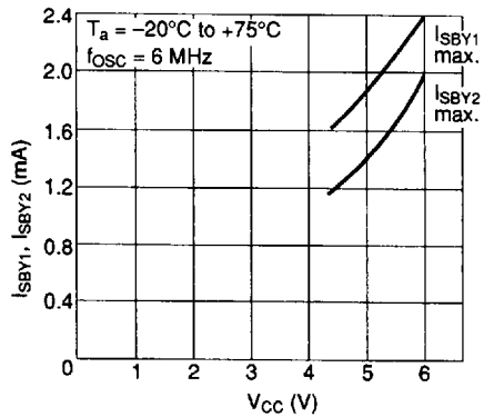
I_{\text{SBY1}}, I_{\text{SBY2}} vs. V_{\text{CC}} characteristics (crystal and ceramic oscillator)
