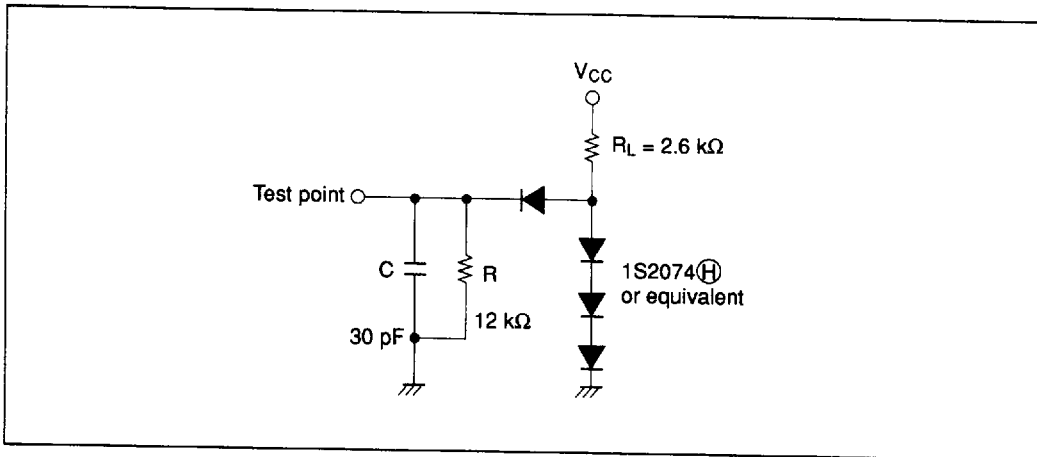
Figure 29 Timing Load Circuit
